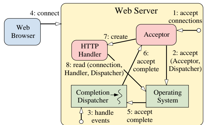
Figure 5: Client connects to a Proactor-based Web Server
