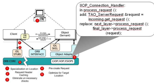
Figure 7. FOCUS: Capturing Specialization Rules
