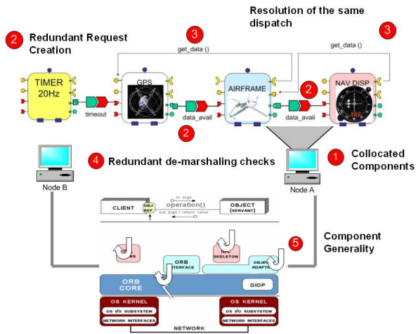
Figure 3. BasicSP Specialization Points
