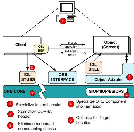
Figure 6. FOCUS: Specialization Identification
