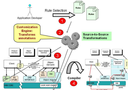
Figure 9. FOCUS: Transformation Process
