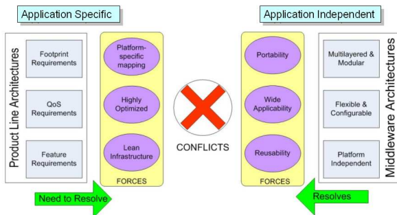
Figure 1. Application-specific vs. Application-independent Dimensions of PLAs and Middleware
