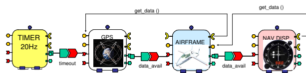
Figure 2. BasicSP Application Scenario
