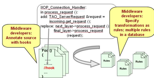
Figure 8. FOCUS: Middleware Annotation
