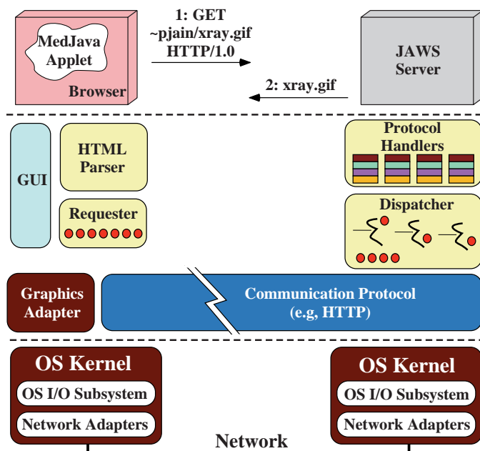
Figure 4. Architecture of MedJava and JAWS
