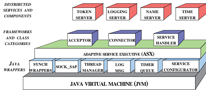
Figure 6. The Java ACE Framework
