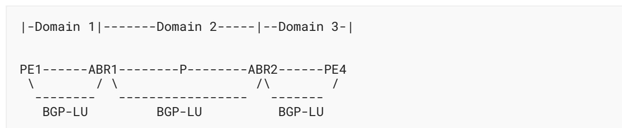
Figure 2: Inter-Domain Networks with Multiple IGPs
