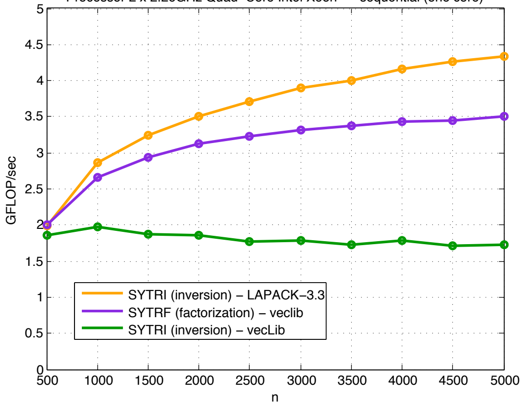
LDLT Inversion (DSYTRI), VecLib Processor 2 x 2.26GHz Quad-Core Intel Xeon -- sequential (one core)
