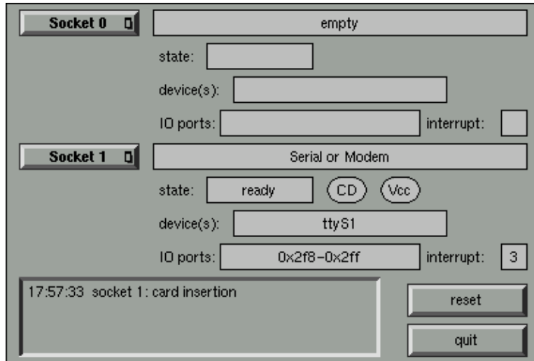
Figure 12-1. Screenshot of cardinfo
